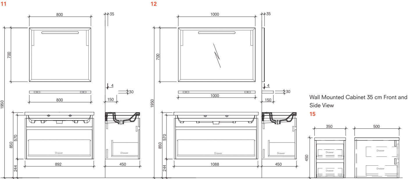
90 cm Set Front and Side View (Illuminated Mirror + Shelf) 110 cm Set Front and Side View (Illuminated Mirror + Shelf)
