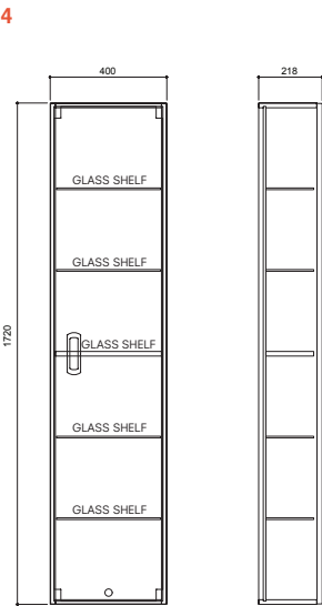
Tall Cabinet 40 cm Front and Side Views
