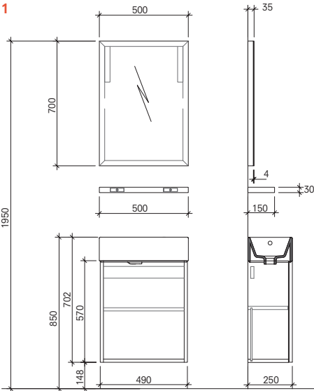
50 cm Set Front and Side View
