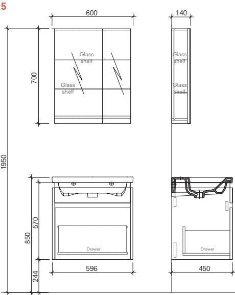
60 cm Set Front and Side View (Mirror Cabinet (Unilluminated))
