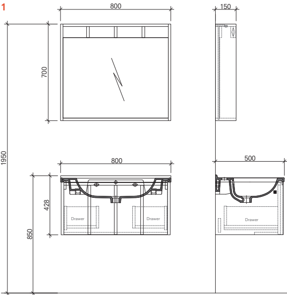
80 cm Set Front and Side View
