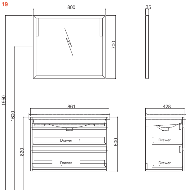
90 cm Set With Drawers Front and Side View (Plain Mirror)
