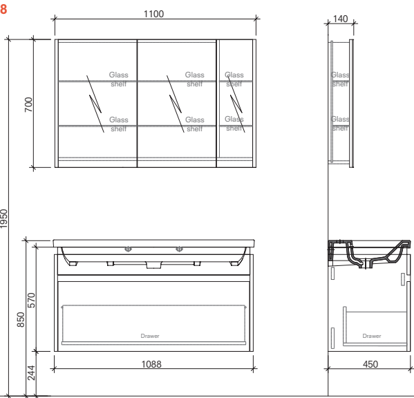
110 cm Set Front and Side View (Mirror Cabinet (Unilluminated))
