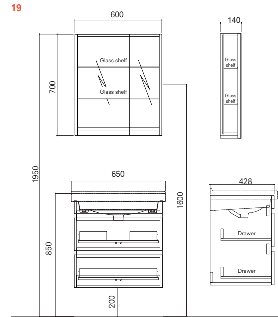
65 cm Set With Drawers Front and Side View (Mirror Cabinet (Unilluminated))
