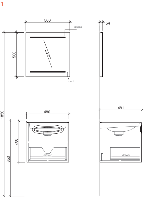
48 cm Set Front and Side View (with shelf)
