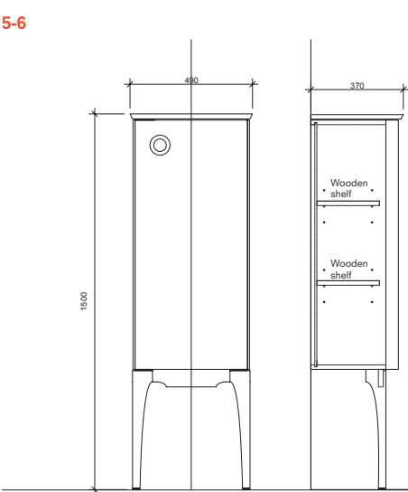
Tall Cabinet 50 cm Front and Side View
