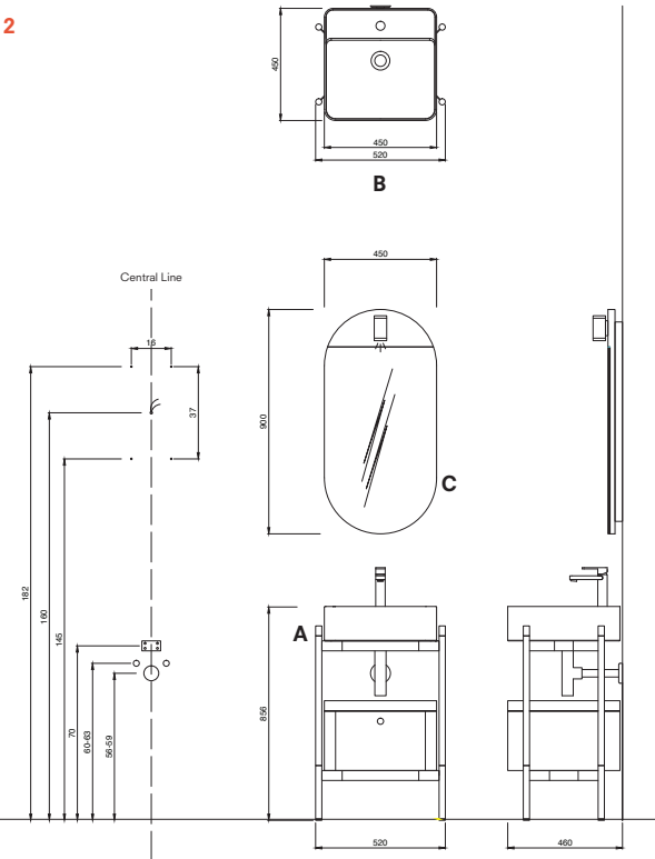
Square Set Front, Side Views and Installation Hole Sizes
