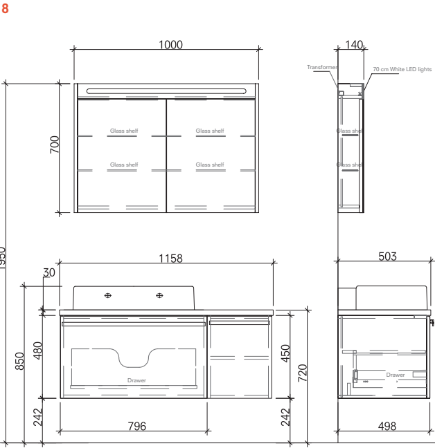
115 cm Set Left Washbasin Front and Side View
