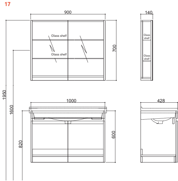
100 cm Set With Door Front and Side View (Mirror Cabinet (Unilluminated))
