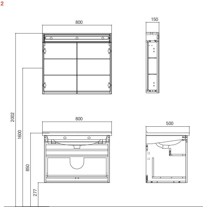
80 cm Set Front and Side Views
