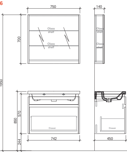
75 cm Set Front and Side View (Mirror Cabinet (Unilluminated))
