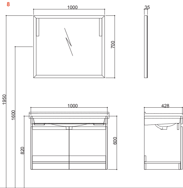
100 cm Set With Door Front and Side View (Plain Mirror)
