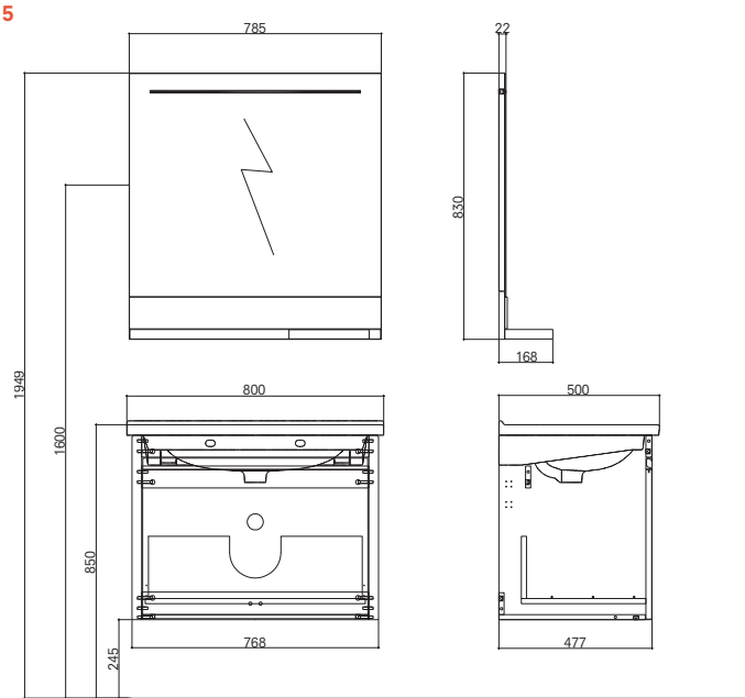
80 cm Set Front and Side Views
