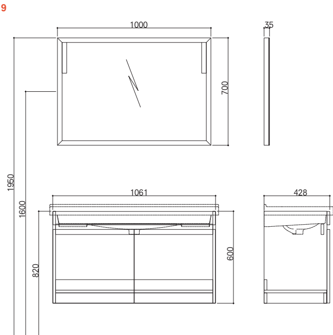
110 cm Set With Door Front and Side View (Plain Mirror)
