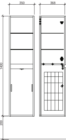
Tall Cabinet 35 cm Front and Side View (With basket)
