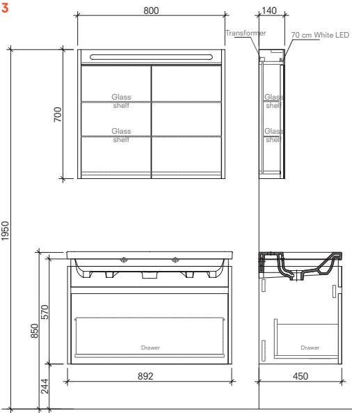
90 cm Set Front and Side View (Illuminated Mirror Cabinet)
