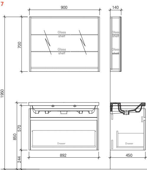
90 cm Set Front and Side View (Mirror Cabinet (Unilluminated))
