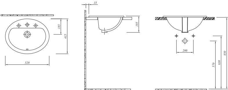
52x41,5 cm Central tap hole, With overflow hole
