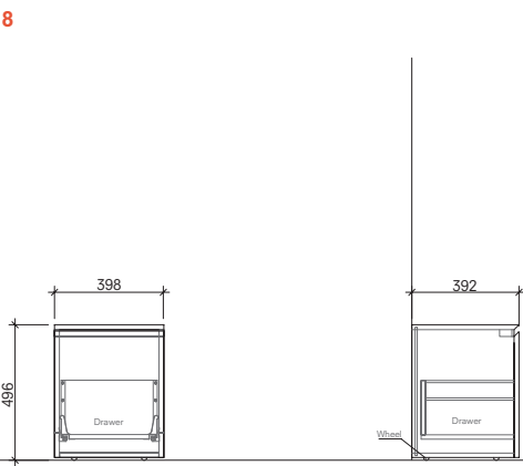
Wheeled Floor Module 40 cm Front and Side View
