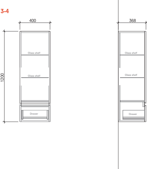
Lower Cabinet 40 cm Front and Side View
