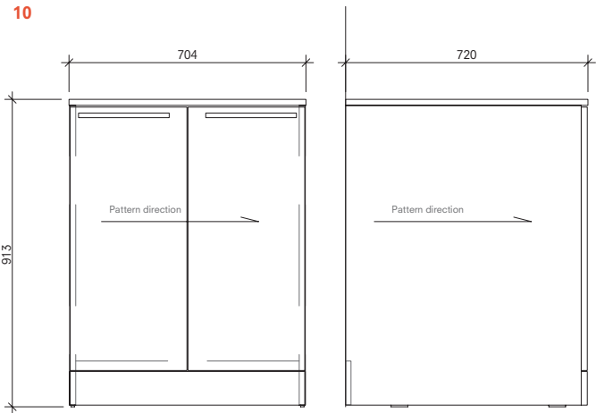
Washing Machine Lower Cabinet 70 cm Front and Side View
