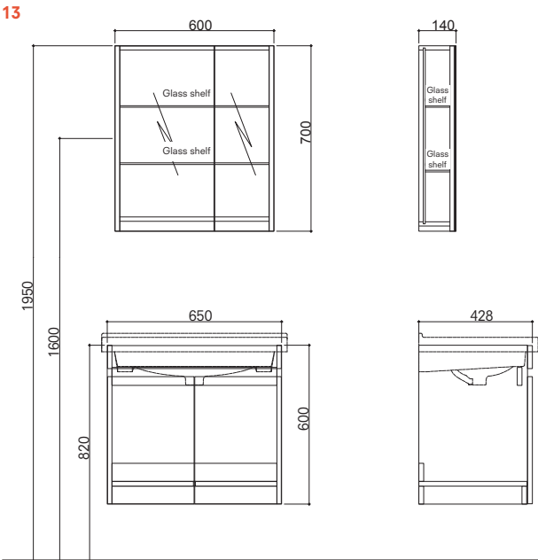
65 cm Set With Door Front and Side View (Mirror Cabinet (Unilluminated))
