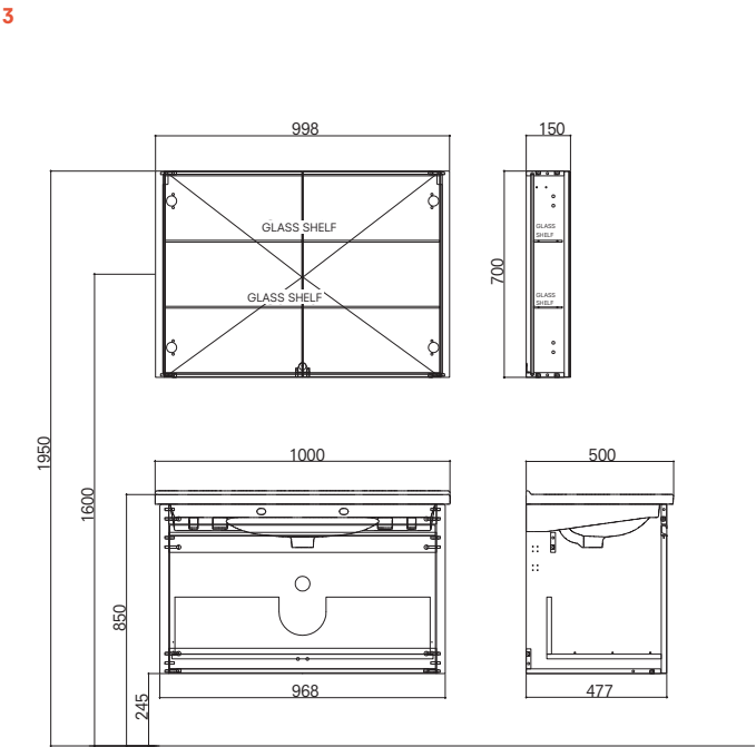
100 cm Set Front and Side Views
