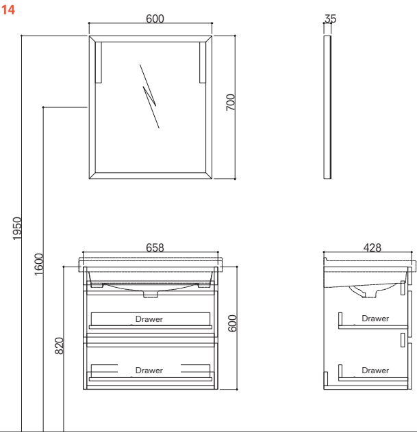
70 cm Set With Drawers Front and Side View (Plain Mirror)
