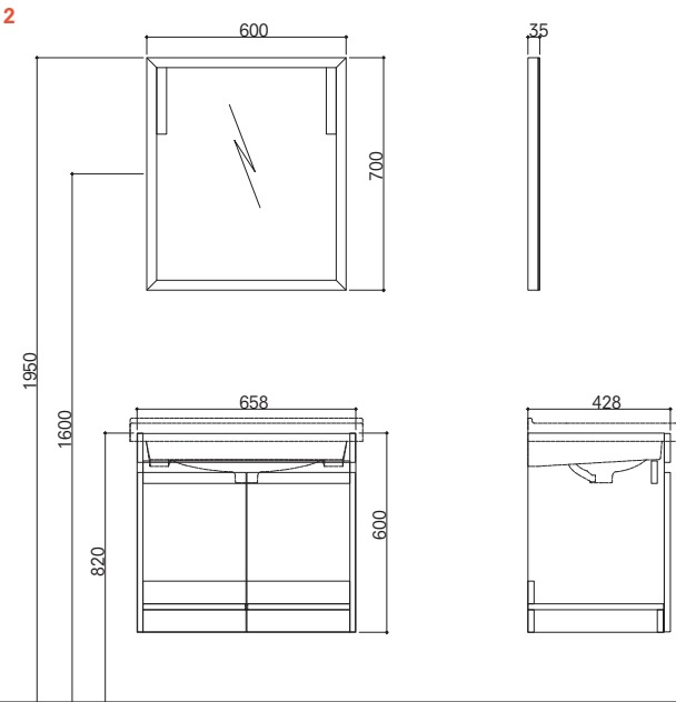
70 cm Set With Door Front and Side View (Plain Mirror)
