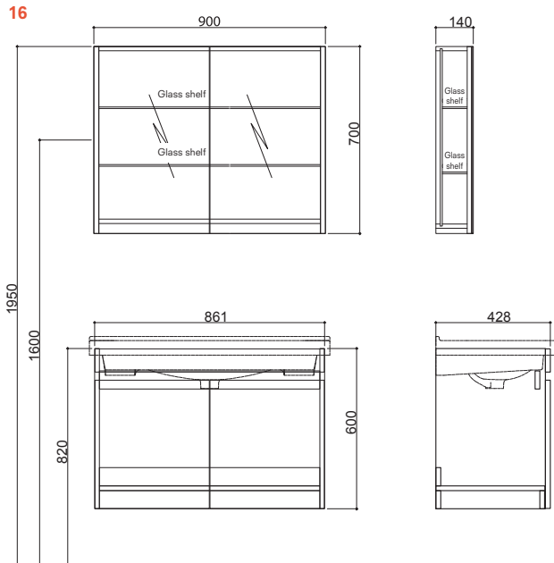
90 cm Set With Door Front and Side View (Mirror Cabinet (Unilluminated))
