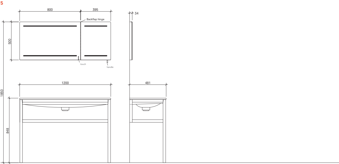
120 cm Set (with Glass Shelf) Front and Side View
