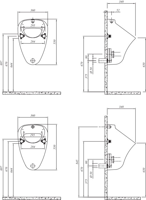
55x36 cm Concealed outlet
