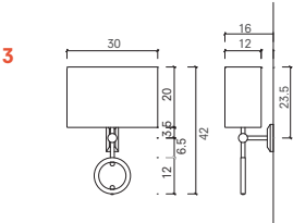
Fabric Wall Light Front and Side View
