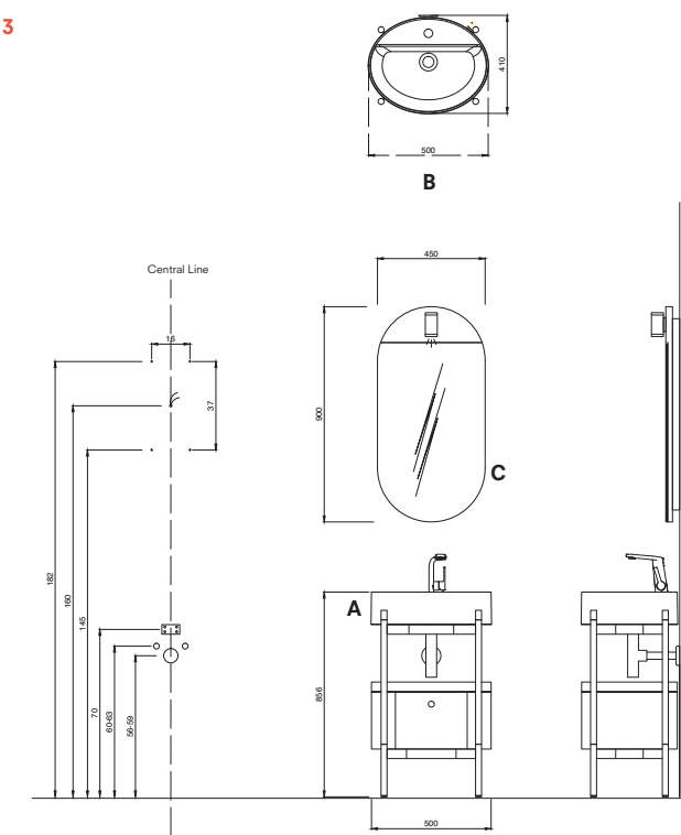
Ellipse Set Front, Side Views and Installation Hole Sizes
