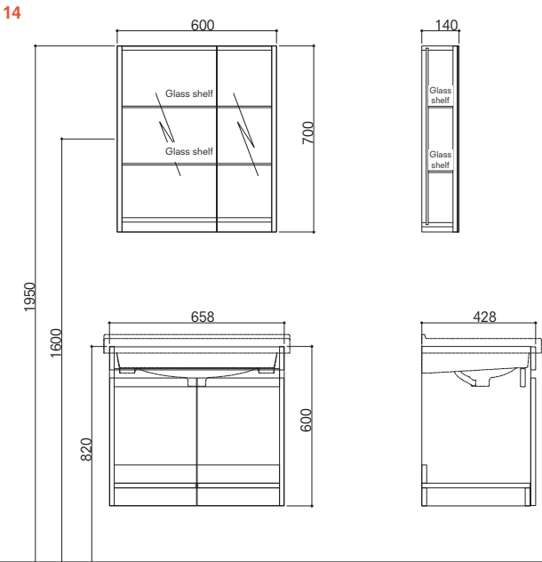
70 cm Set With Door Front and Side View (Mirror Cabinet (Unilluminated))
