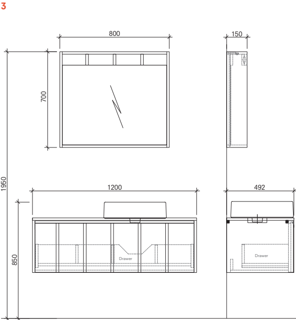
120 cm Set (80 cm Mirror Cabinet) Front and Side View
