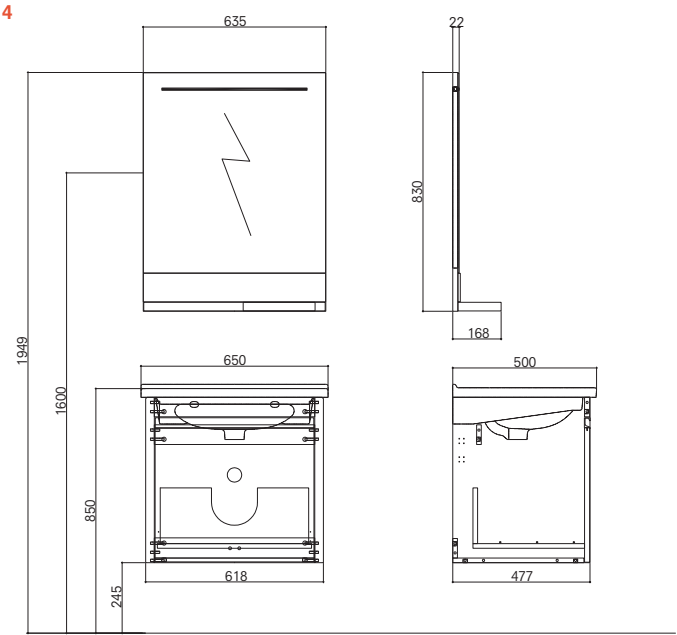
65 cm Set Front and Side Views
