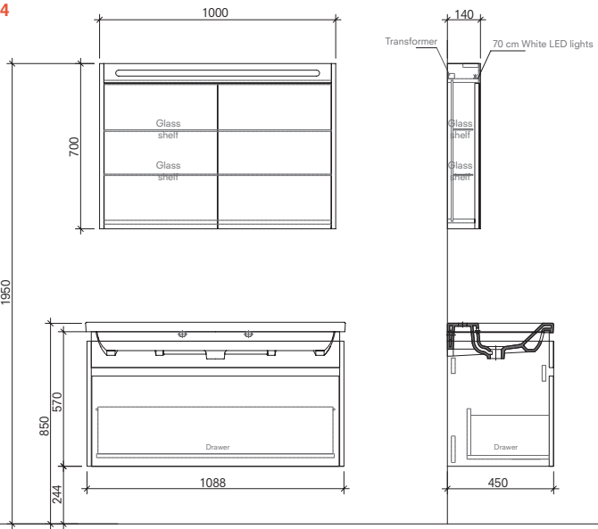
110 cm Set Front and Side View (Illuminated Mirror Cabinet)
