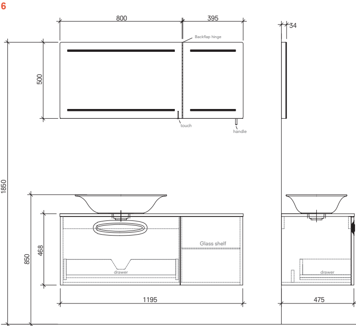
120 cm Set Bowl Washbasin (Left) Front and Side View
