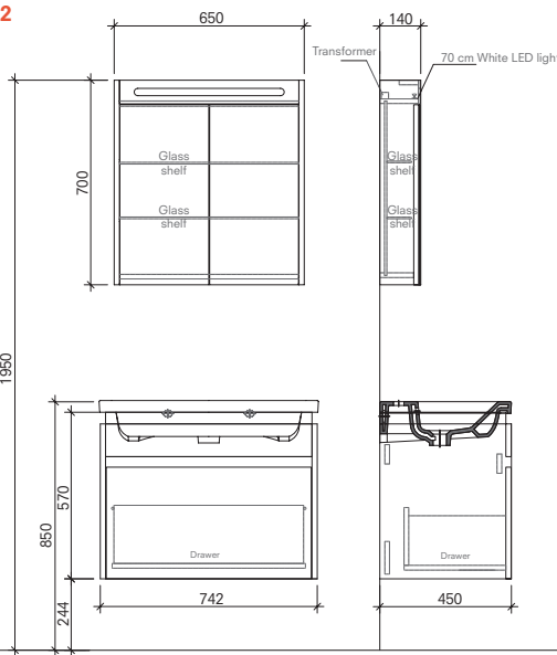
75 cm Set Front and Side View (Illuminated Mirror Cabinet)
