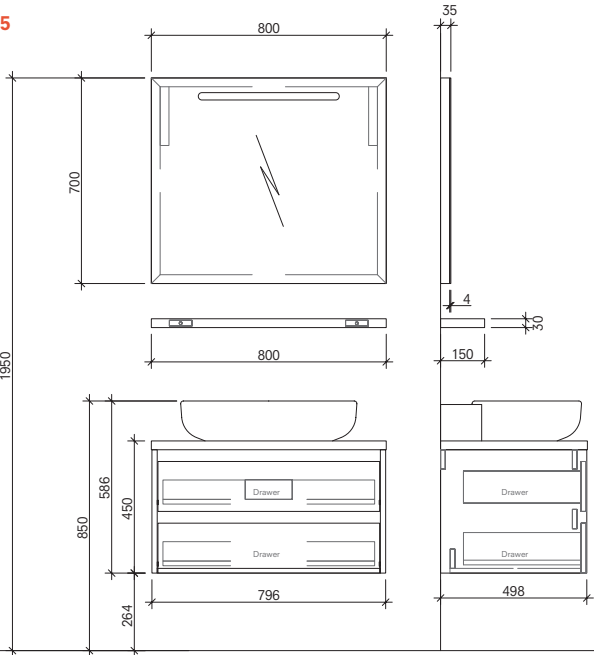
80 cm Set Front and Side View (Illuminated Mirror Cabinet + Shelf)
