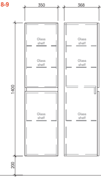
Tall Cabinet 35 cm Right/Left (with Basket) Front and Side View
