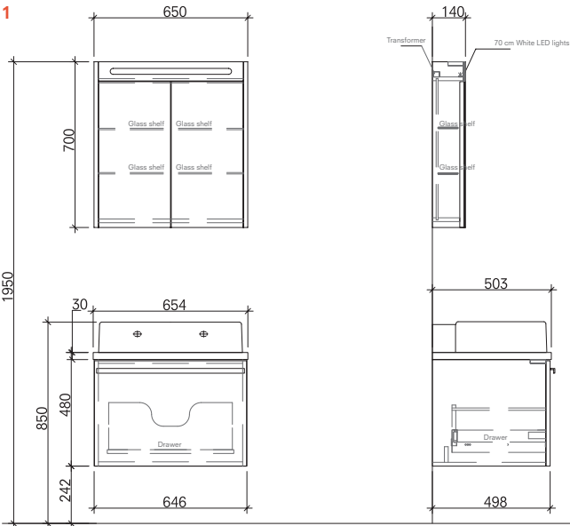
65 cm Set Tall Front and Side View
