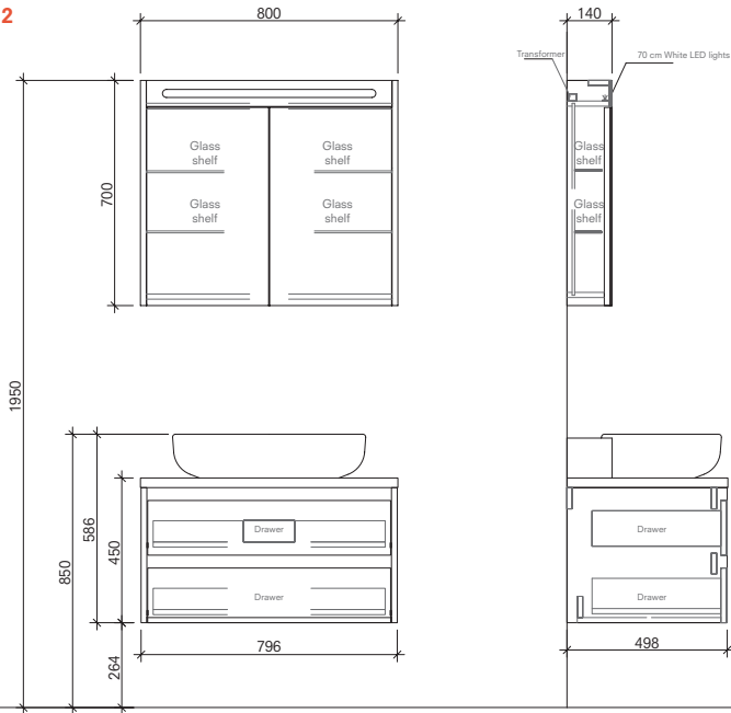
80 cm Set Front and Side View (Illuminated Mirror Cabinet)
