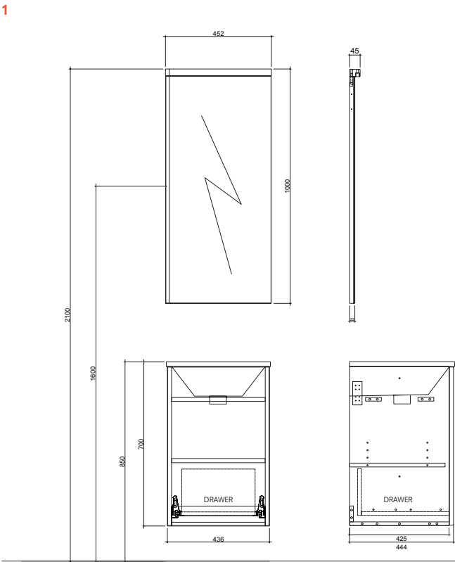
45 cm Set Front and Side Views
