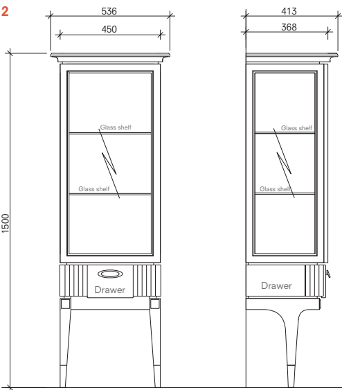
Tall Cabinet 45 cm Front and Side View
