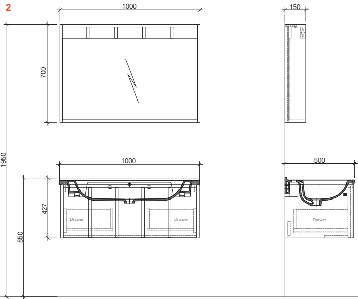
100 cm Set Front and Side View
