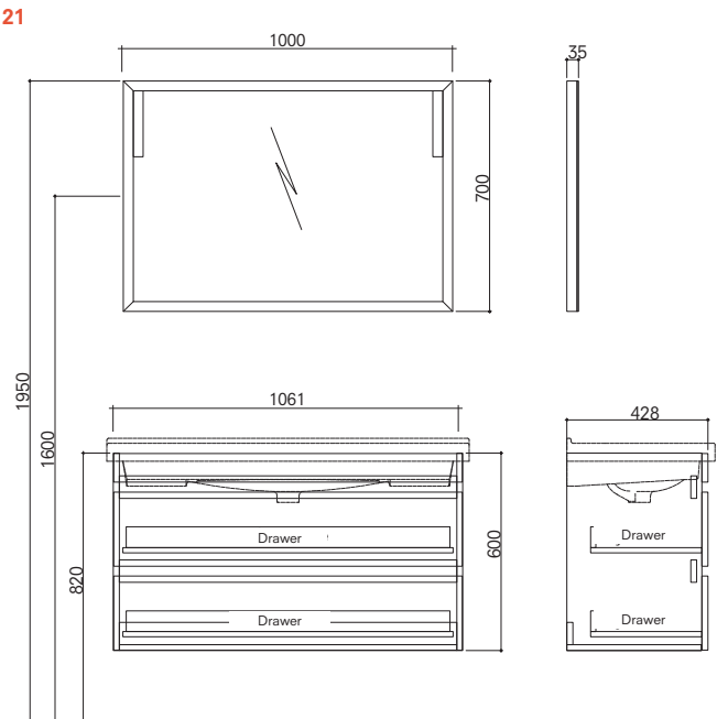
110 cm Set With Drawers Front and Side View (Plain Mirror)
