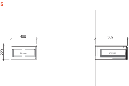
Floor Module with Integrated Damper 40 cm Front and Side View
