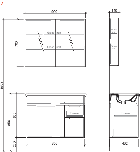
90 cm Set Front and Side View
