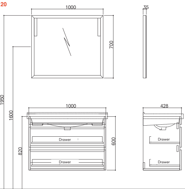
100 cm Set With Drawers Front and Side View (Plain Mirror)
