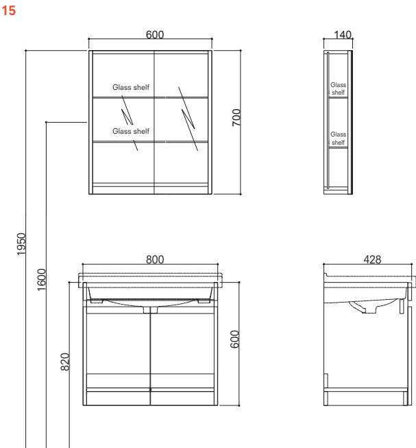
80 cm Set With Door Front and Side View (Mirror Cabinet (Unilluminated))
