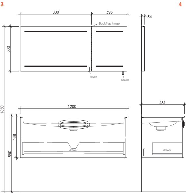
120 cm Set Front and Side View (with shelf)
