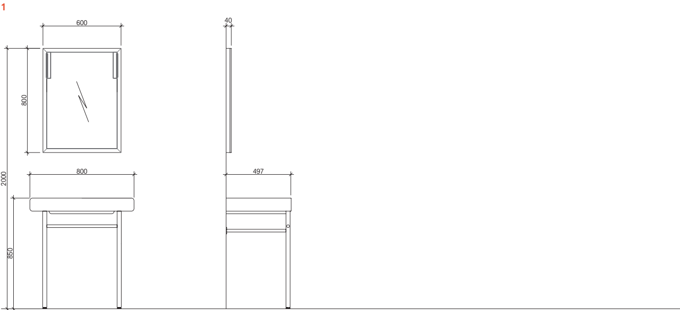
Lazuli Fold Set Front and Side View
