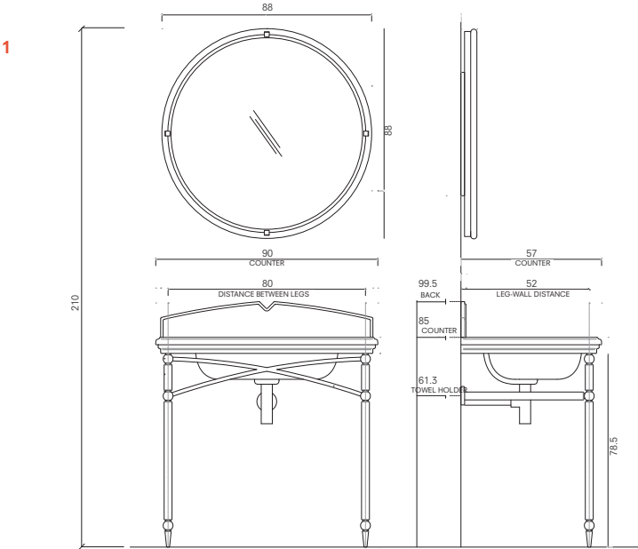
90 cm Set Front and Side View
