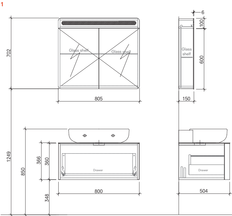
80 cm Set Front and Side View
