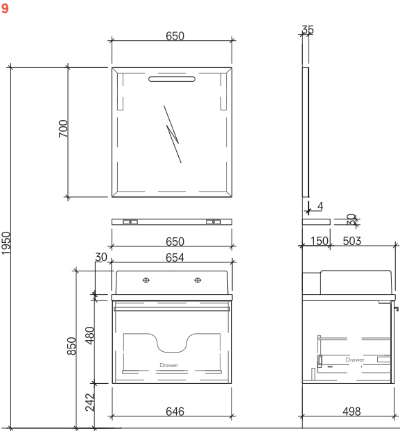
65 cm Set Tall Front and Side View
