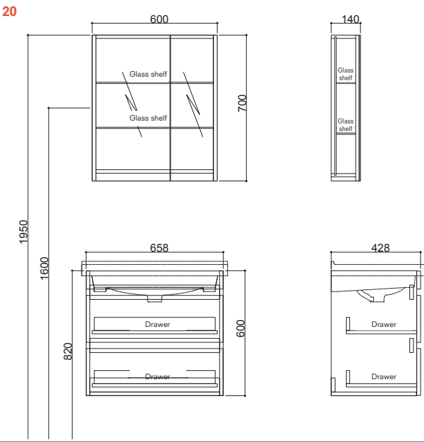
70 cm Set With Drawers Front and Side View (Mirror Cabinet (Unilluminated))
