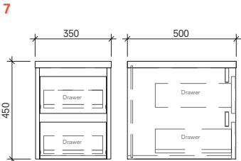
Wall Mounted Cabinet 35 cm Front and Side View
