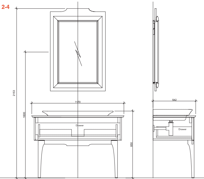
115 cm Set Front and Side View
