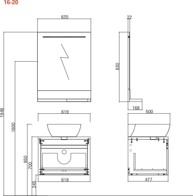
65 cm Set Bowl Washbasin
