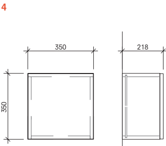
Wall Mounted Cabinet h: 35 cm Front and Side View
