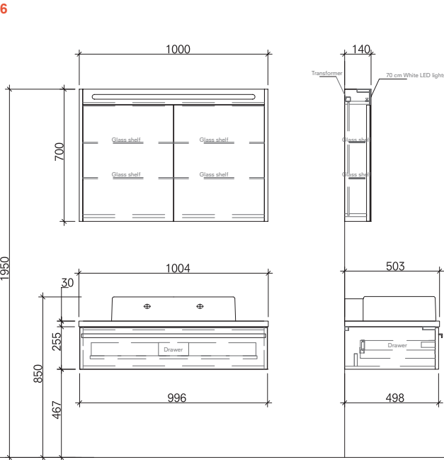
100 cm Set Short Front and Side View
