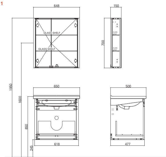
65 cm Set Front and Side Views
