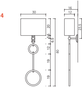
Fabric Wall Light Front and Side View (With Towel Holder)
