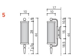
Glass Wall Light Front and Side View
