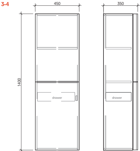
45 cm Tall Cabinet Front and Side View (Left/Right)
