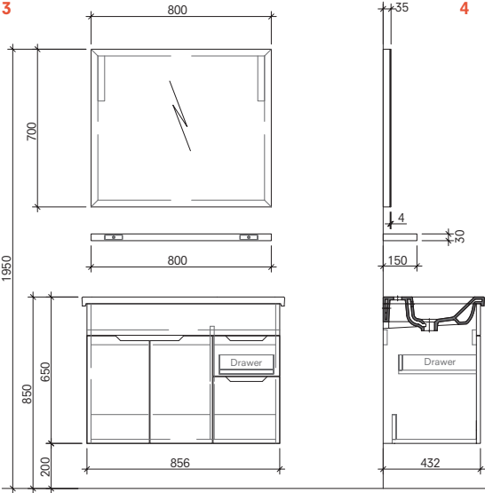
90 cm Set Front and Side View
