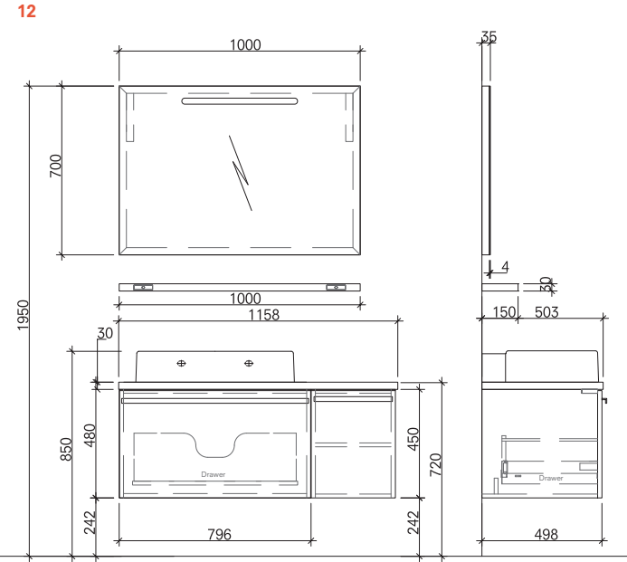
115 cm Set Tall Front and Side View
