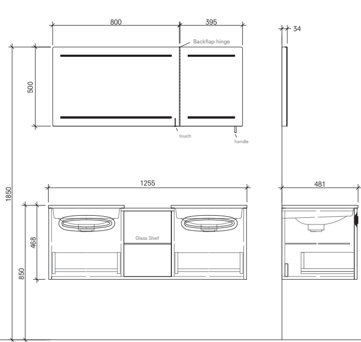
125 cm Set Double Washbasin (with shelf) Front and Side View
