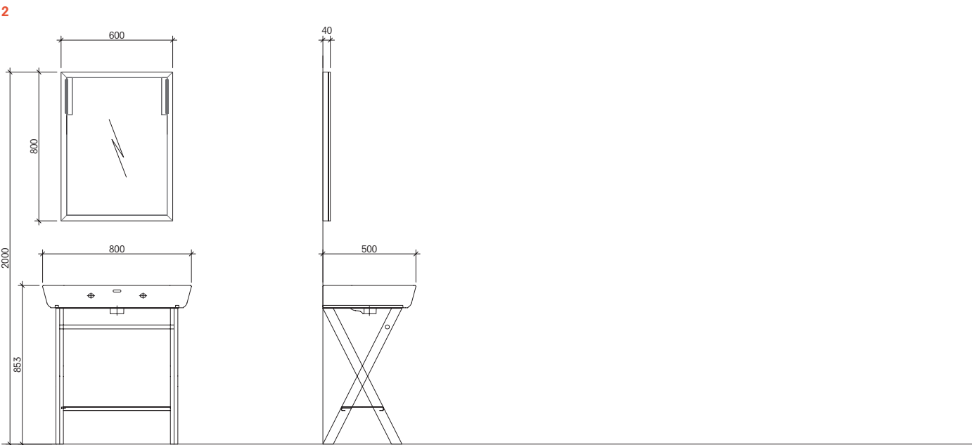
Lazuli Nordic Set Front and Side View
