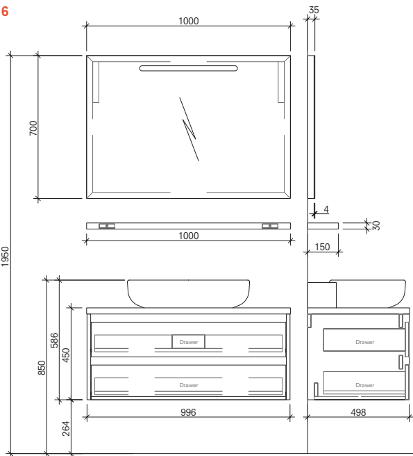
100 cm Set Front and Side View (Illuminated Mirror Cabinet + Shelf)
