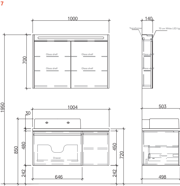
100 cm Set Left Washbasin Front and Side View
