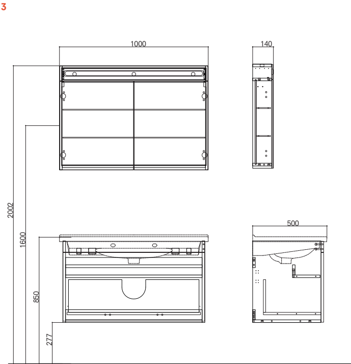
100 cm Set Front and Side Views
