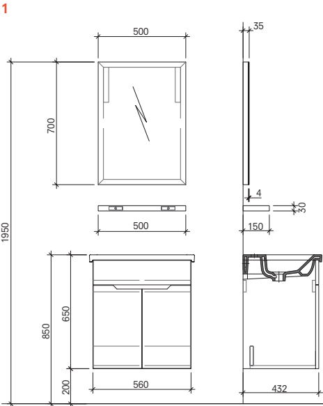
60 cm Set Front and Side View
