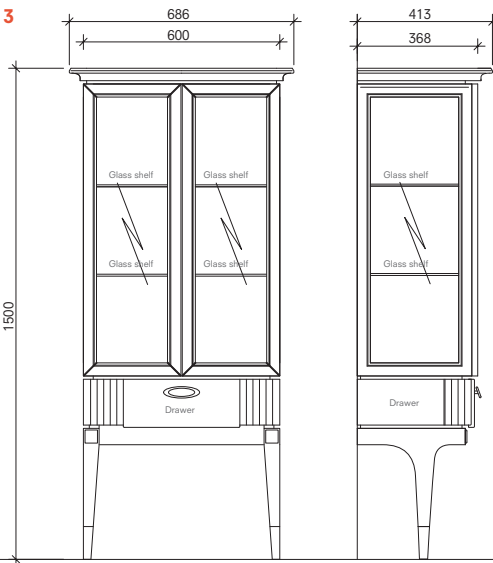
Tall Cabinet 60 cm Front and Side View
