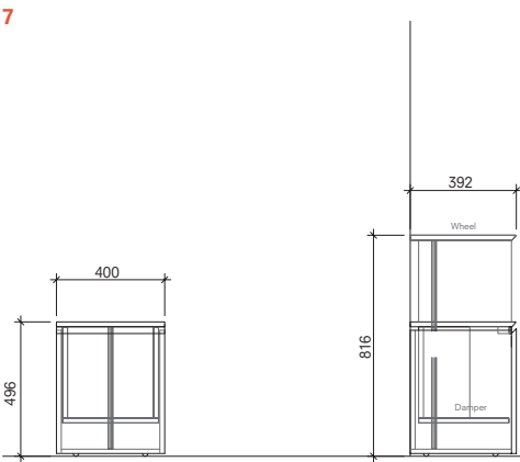
Floor Module with Integrated Damper 40 cm Front and Side View
