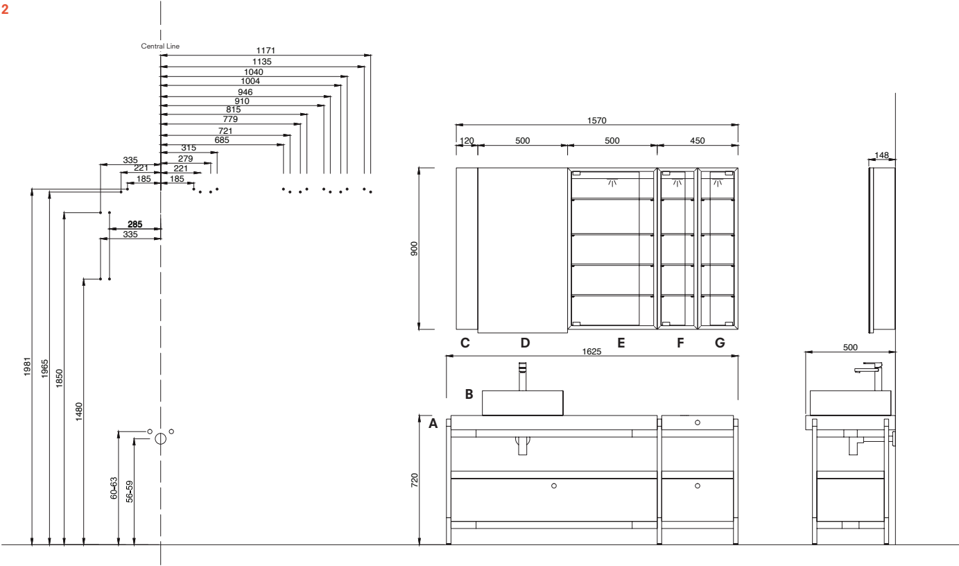
165 cm Set Front, Side Views and Installation Hole Sizes
