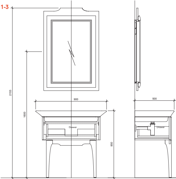
90 cm Set Front and Side View
