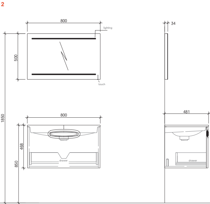
80 cm Set Front and Side View (with shelf)
