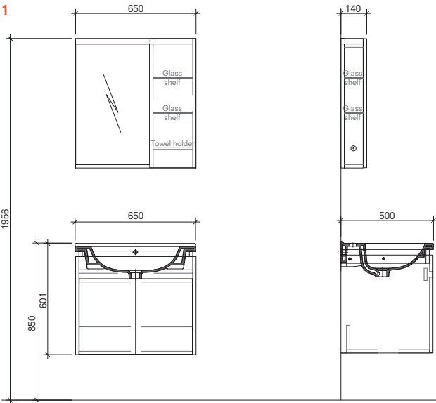
65 cm Set Front and Side View
