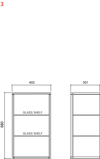
Lower Side Module with Glass Shelf 40 cm
