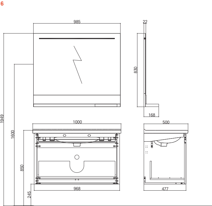
100 cm Set Front and Side Views
