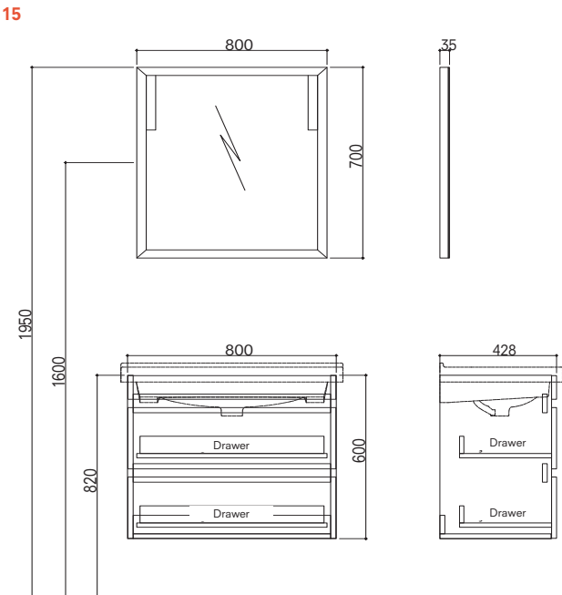
80 cm Set With Drawers Front and Side View (Plain Mirror)
