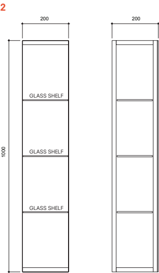
Open Shelf Mirrored Top Module 20 cm Front and Side Views
