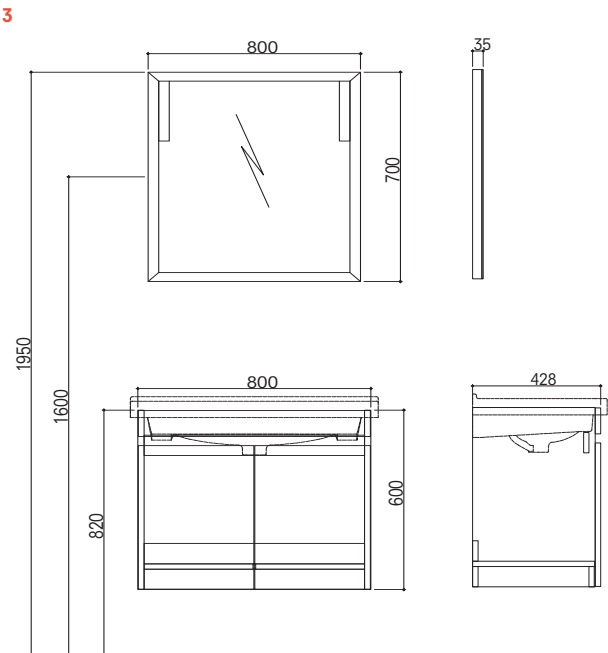
80 cm Set With Door Front and Side View (Plain Mirror)
