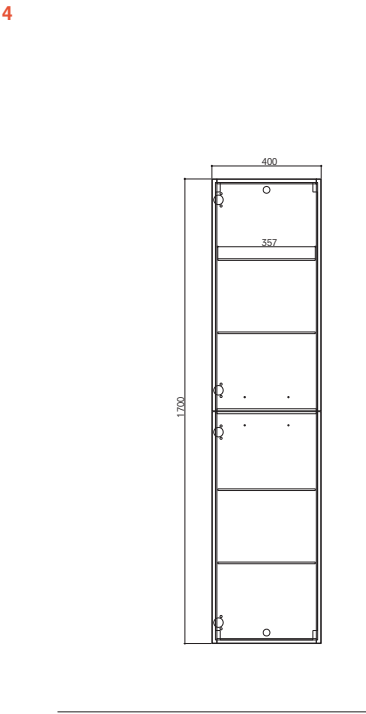
Tall Cabinet 35 cm (Right/Left) Side View
