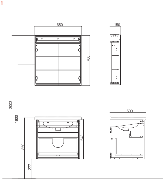
65 cm Set Front and Side Views
