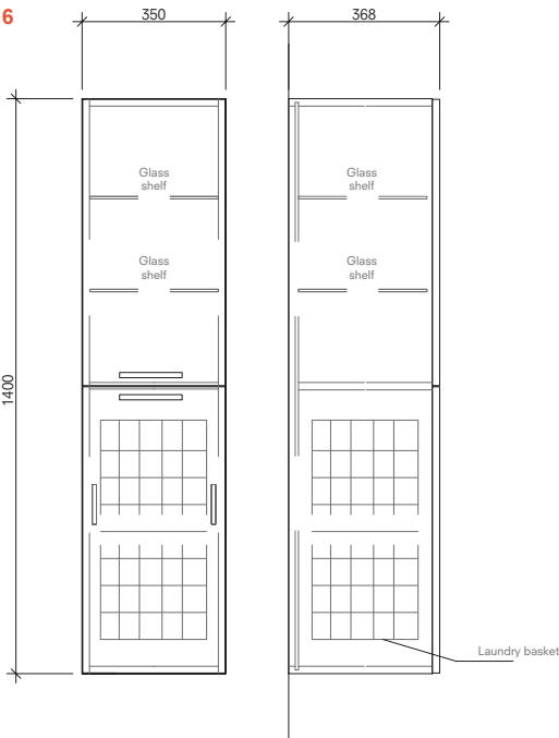
Tall Cabinet 35 cm Right/Left (with Basket) Front and Side View
