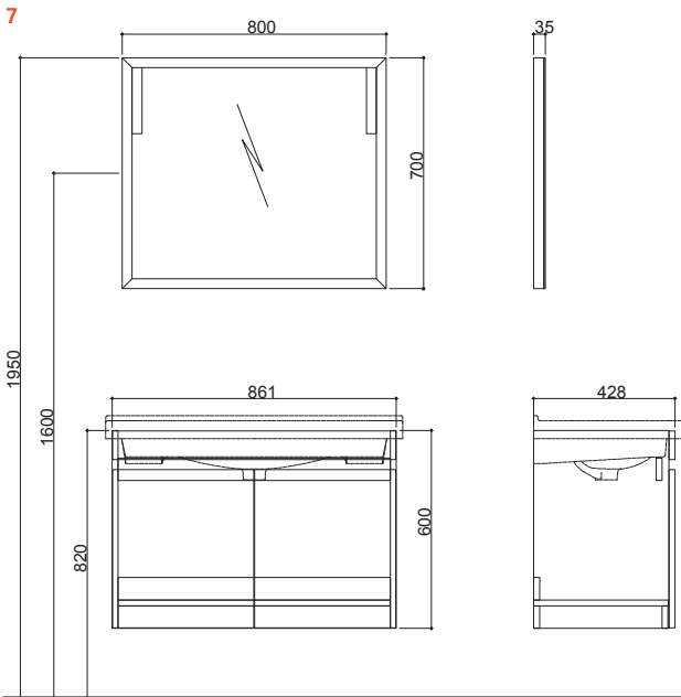
90 cm Set With Door Front and Side View (Plain Mirror)
