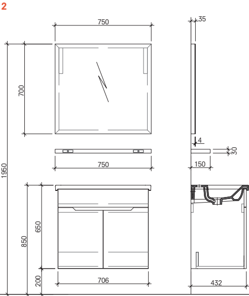
75 cm Set Front and Side View
