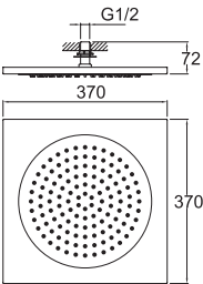
RAIN SHOWER HEAD [37cmx37cm]
