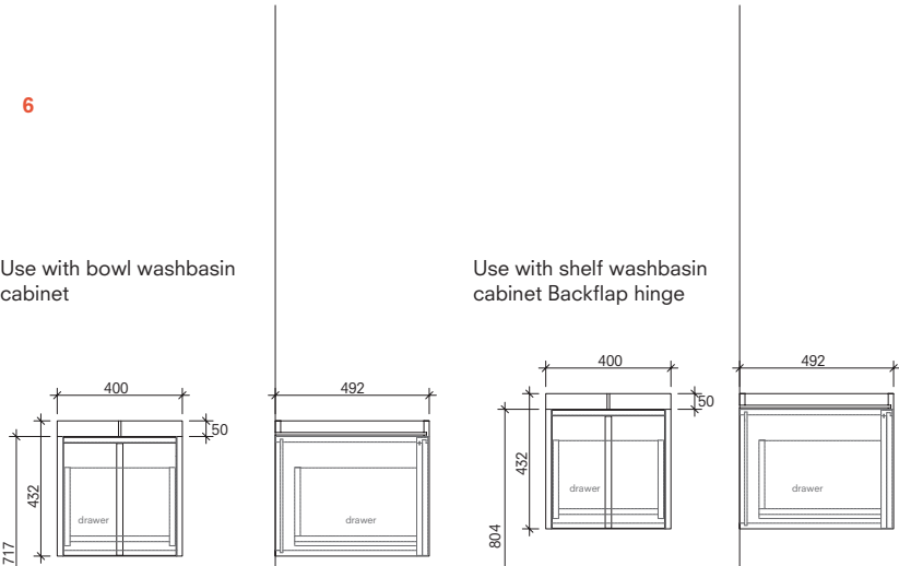
40 cm Lower Cabinet Front and Side View
