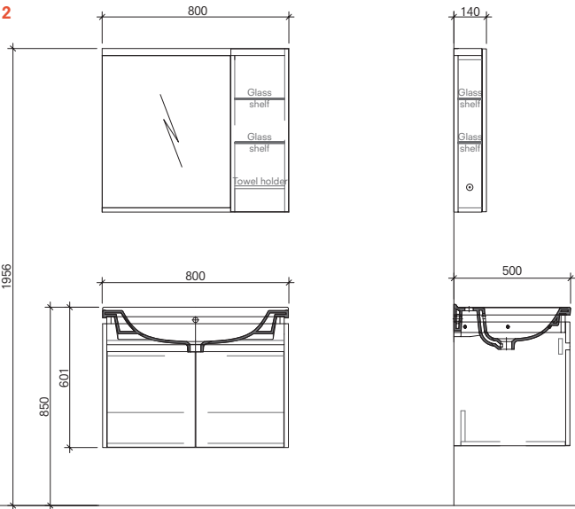
80 cm Set Front and Side View
