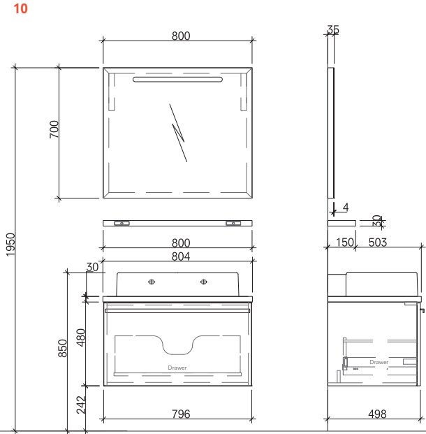
80 cm Set Tall Front and Side View
