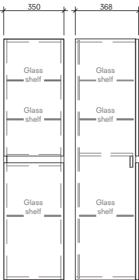
Tall Cabinet 35 cm Front and Side View (Not basket)
