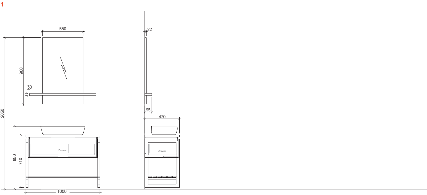
100 cm Front and Side View
