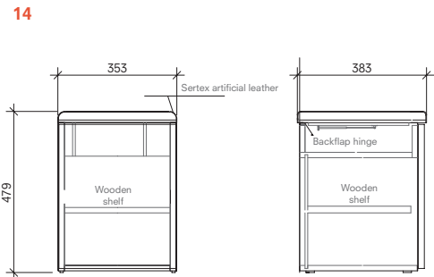
Ottoman with Storage 35 cm Front and Side View
