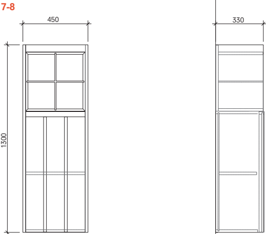
Tall Cabinet 40 cm Front and Side View
