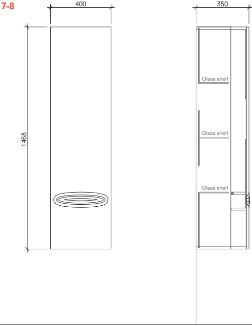
Tall Cabinet 40 cm (Left-Right) Front and Side View
