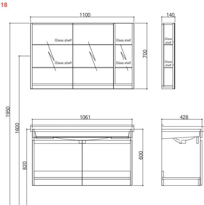
110 cm Set With Door Front and Side View (Mirror Cabinet (Unilluminated))
