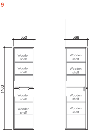
Tall Cabinet Front and Side View
