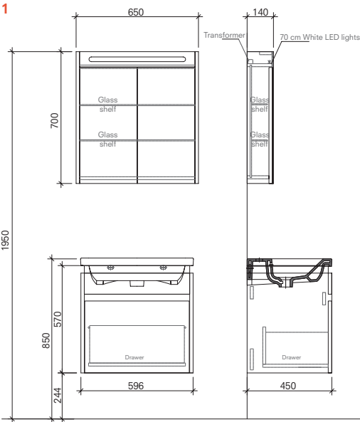
60 cm Set Front and Side View (Illuminated Mirror Cabinet)
