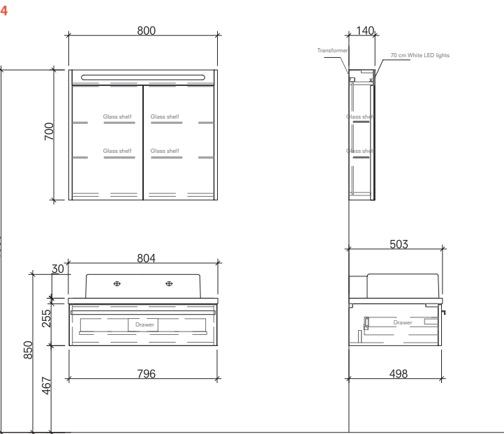
80 cm Set Short Front and Side View
