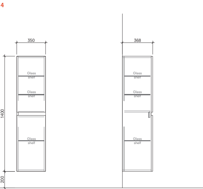
35 cm Tall Cabinet Right/Left Front and Side View
