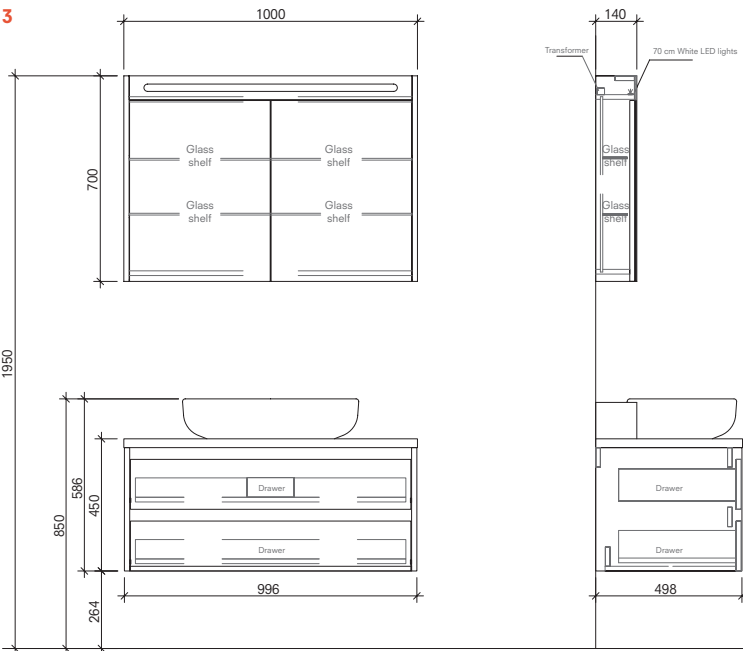
100 cm Set Front and Side View (Illuminated Mirror Cabinet)
