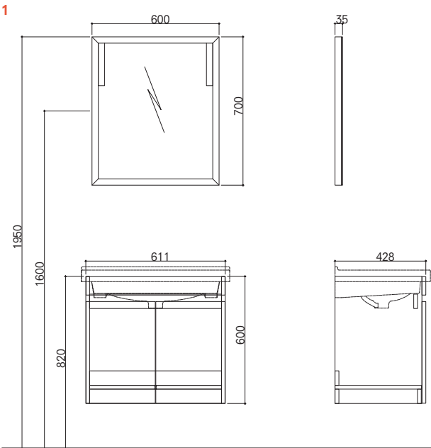
65 cm Set With Door Front and Side View (Plain Mirror)
