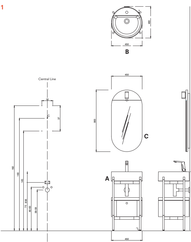
Ellipse Set Front, Side Views and Installation Hole Sizes
