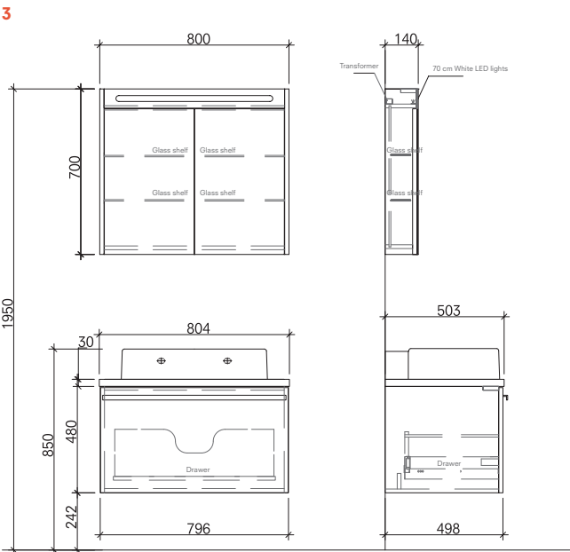
80 cm Set Tall Front and Side View
