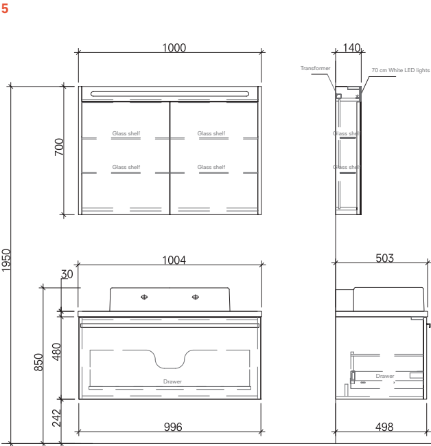
100 cm Set Tall Front and Side View
