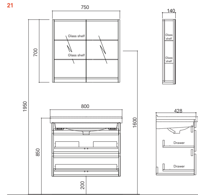
80 cm Set With Drawers Front and Side View (Mirror Cabinet (Unilluminated))
