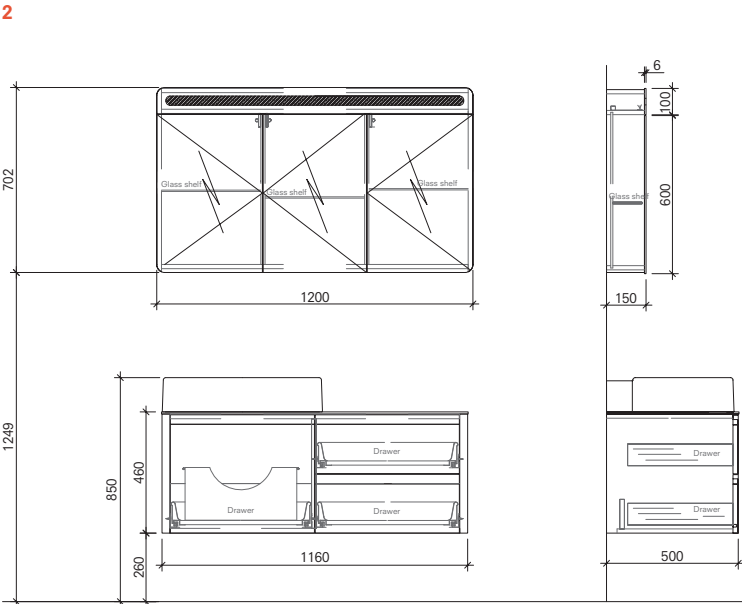
120 cm Set Front and Side View
