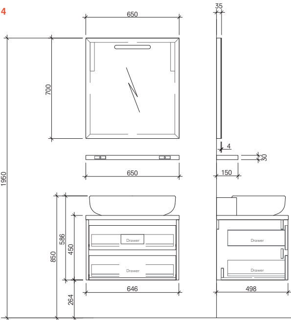
65 cm Set Front and Side View (Illuminated Mirror Cabinet + Shelf)
