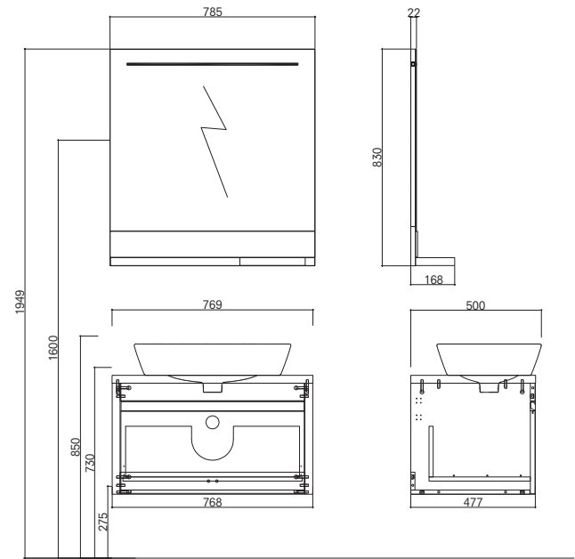
80 cm Set Bowl Washbasin
