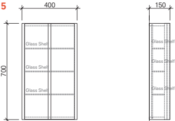
40 cm Upper Side Cabinet Front and Side View
