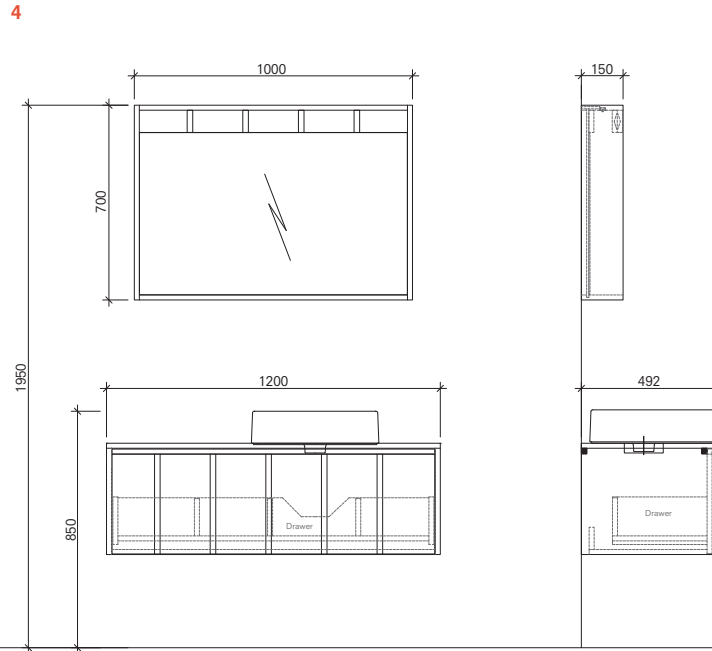
80 cm Set (100 cm Mirror Cabinet) Front and Side View
