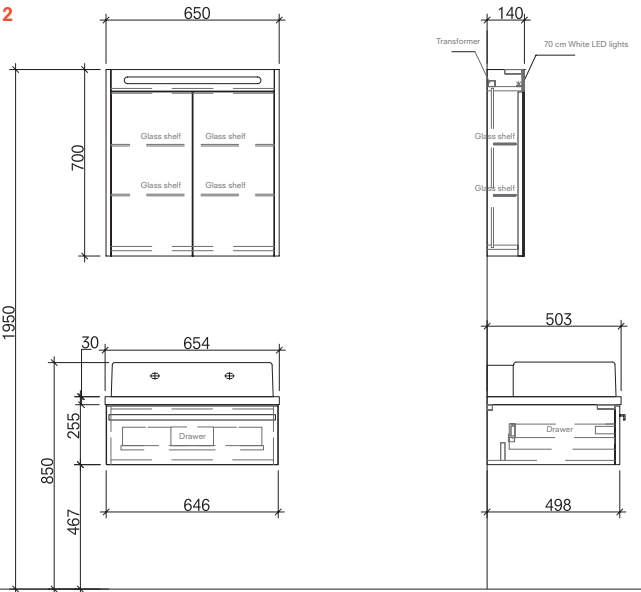
65 cm Set Short Front and Side View
