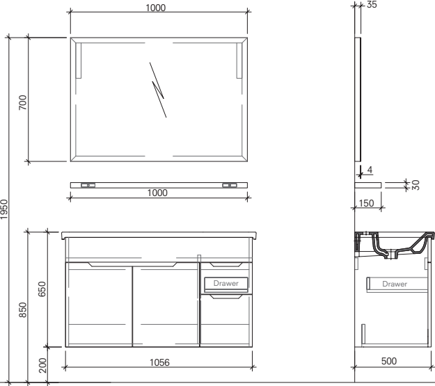
110 cm Set Front and Side View
