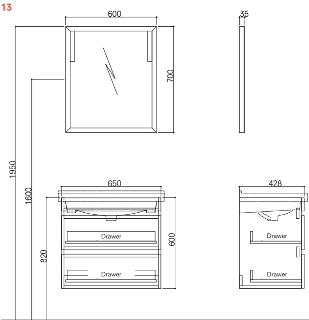
65 cm Set With Drawers Front and Side View (Plain Mirror)
