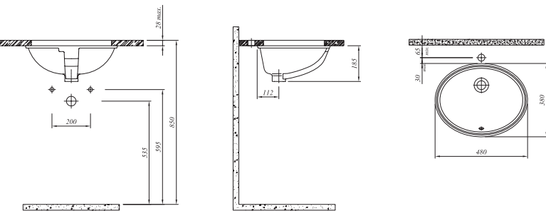
48x38 cm With central tap hole, overflow hole
