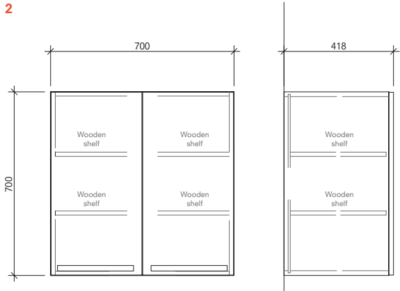
Washing Machine Upper Cabinet 70 cm Front and Side View
