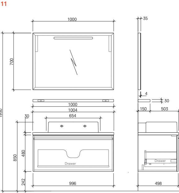
100 cm Set Tall Front and Side View
