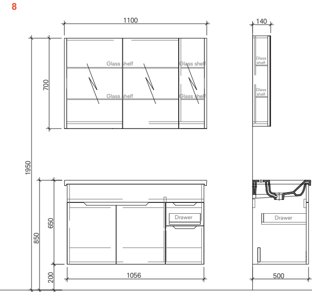
110 cm Set Front and Side View
